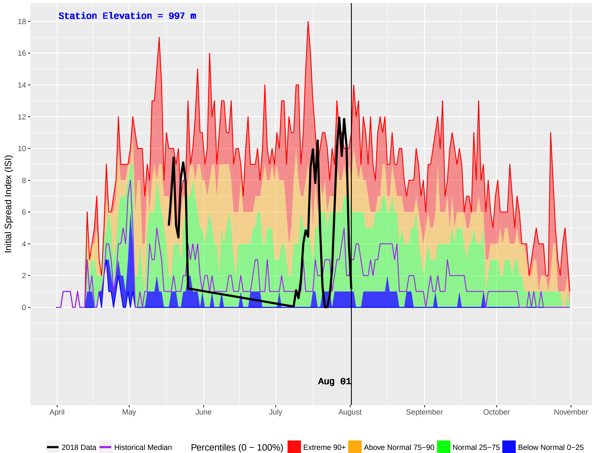
JERRY (190) : Historical (1988–2016) and Current (2018) Daily Initial Spread Index (ISI)
