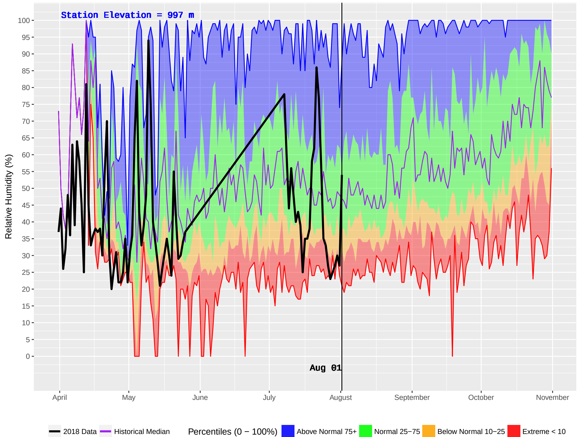
JERRY (190) : Historical (1988–2016) and Current (2018) Daily Relative Humidity
